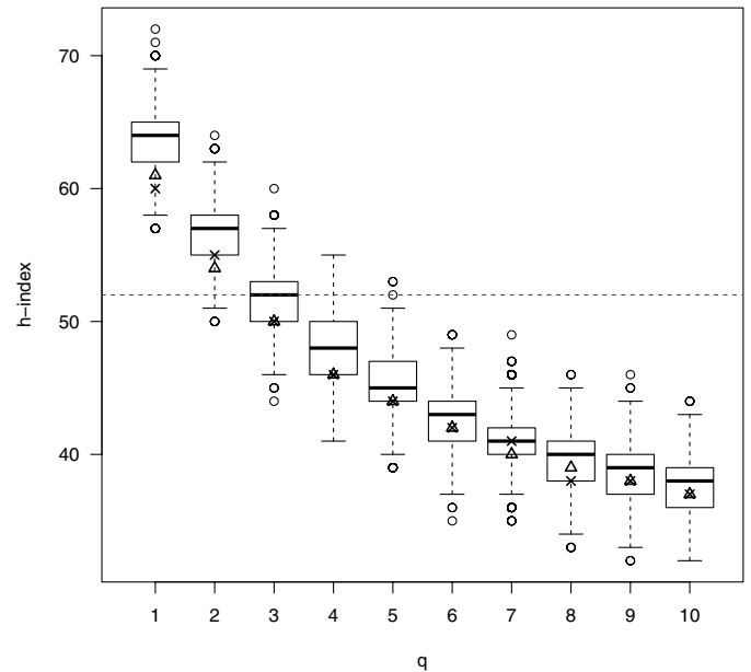
Fig. 1. Boxplots for the distribution of the h -index of Hirsch as estimated via the IC model. Additionally, the h -index computed according to citation vectors obtained via equations (7) and (8) is marked with \Delta and the h -index obtained from averaged citation vectors from the IC model by \times .
