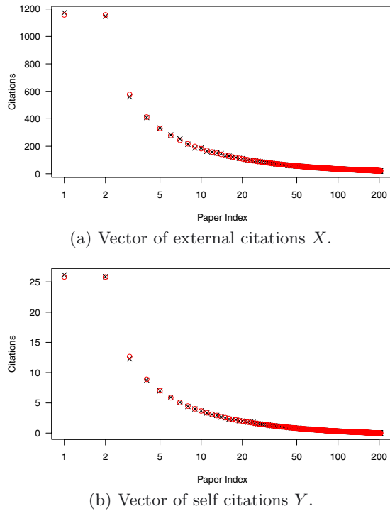
Fig. 2. Step plots of vectors of external X and self citations Y obtained from the IC model, depicted by \times , and equations (7) and (8), depicted by \circ .
