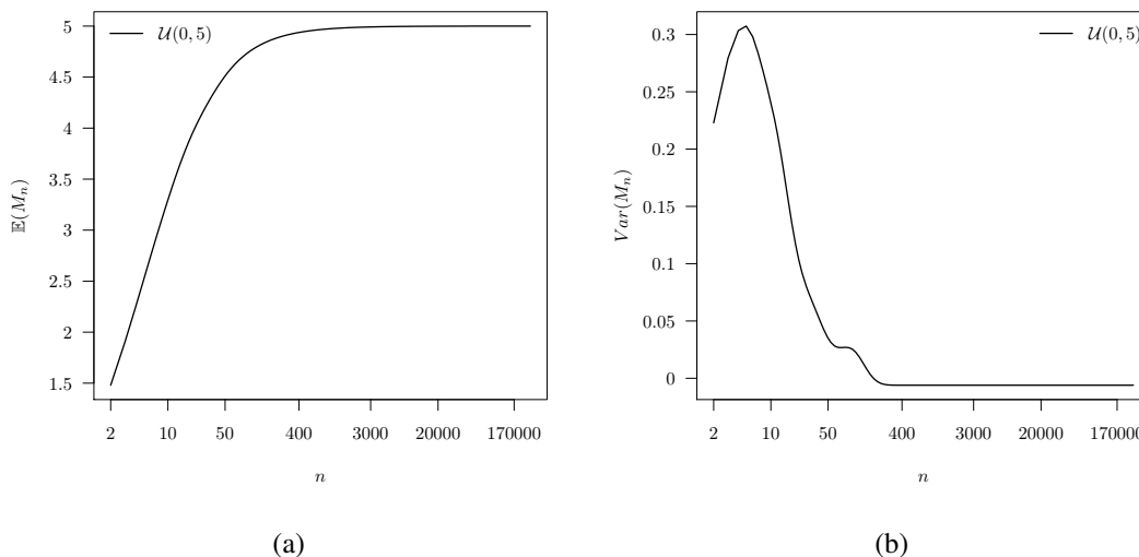
Figure 3: Expected value (a) and variance (b) of OM3 operators for a sample of random variables from the uniform distribution on [0, 5] , as a function of sample length, n .
