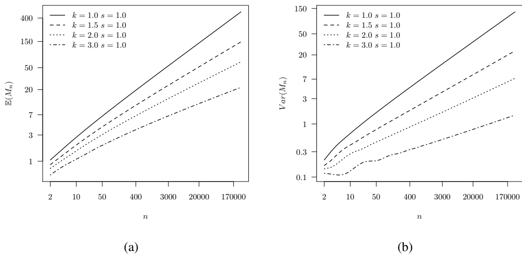
Figure 5: Expected value (a) and variance (b) of OM3 operators for samples of random variables from various Pareto-type II distributions as a function of sample length, n .
