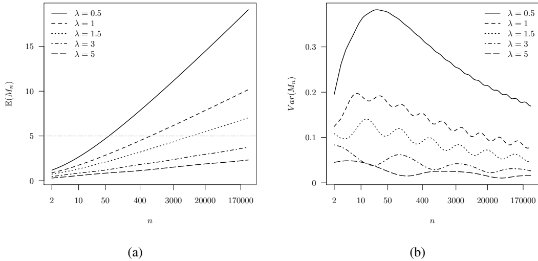
Figure 4: Expected value (a) and variance (b) of OM3 operators for samples of random variables from various exponential distributions as a function of sample length, n .
